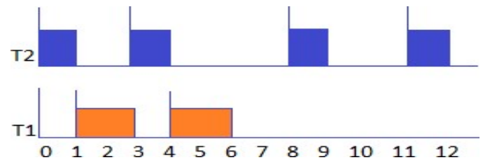
Figure 2: Scheduling example of Rate-Monotonic
